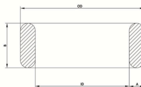
R - Oval Gasket Style
